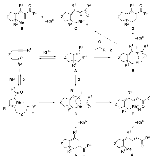
Scheme 3. A possible mechanism for the reaction of enyne 1 with alkene 2 .
