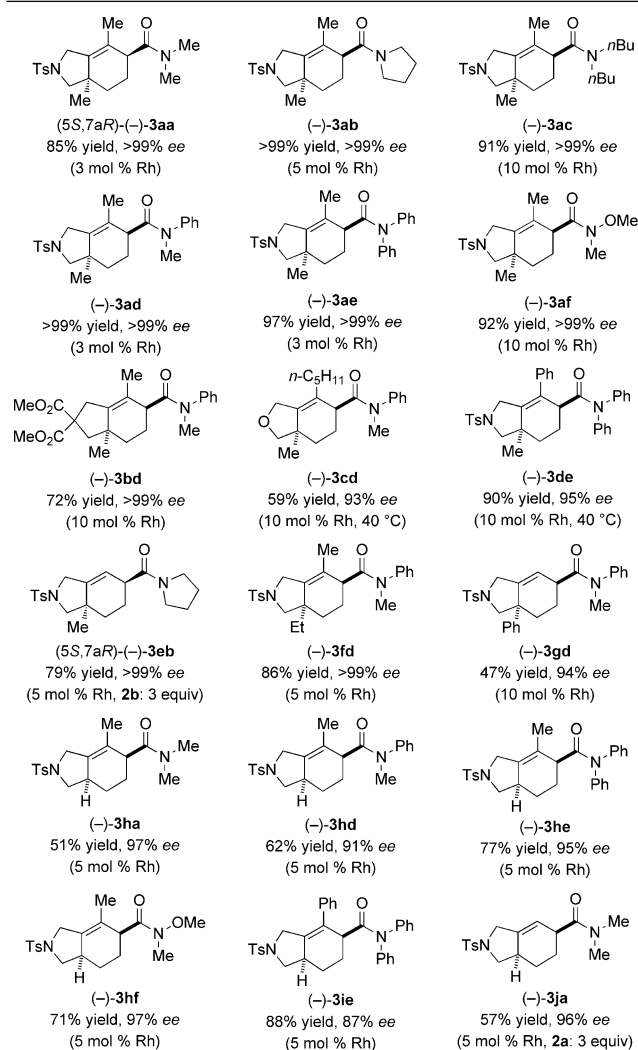
Scheme 2. Rhodium-catalyzed asymmetric [2+2+2] cycloaddition of 1,6-enynes 1a–j with acrylamides 2a–f . Reaction conditions: [Rh(cod) 2 ]BF 4 (0.0060–0.020 mmol), ( R )-H 8 -binap (0.0060–0.020 mmol), 1 (0.20 mmol), 2 (0.22–0.60 mmol), and CH 2 Cl 2 (1.5 mL) were used. Cited yields are of isolated products.
