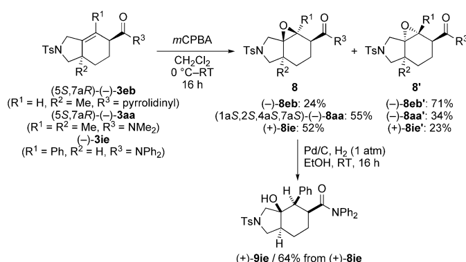
Scheme 6. Oxidative transformations of chiral annulated cyclohexenes 3 .
