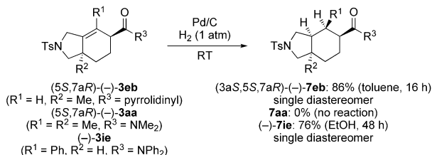
Scheme 5. Reductive transformations of chiral annulated cyclohexenes 3 .
